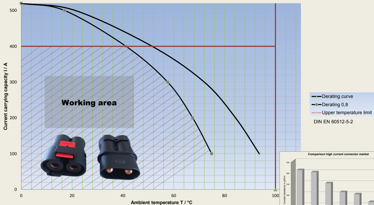
Derating curve - AKNH contact system
